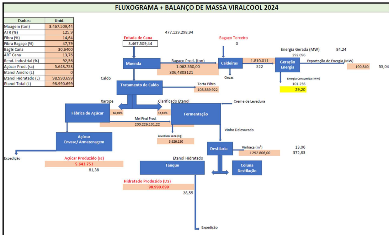
Fluxograma Setor Industrial
